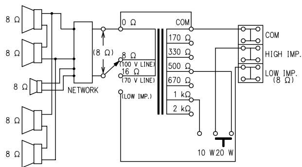
Wiring Diagram
