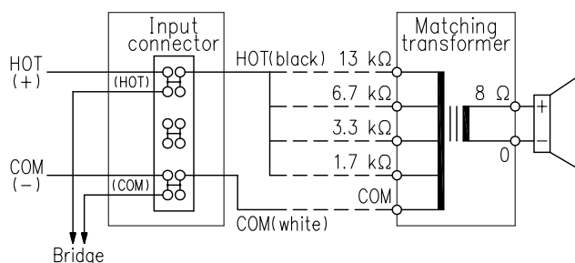
Wiring Diagram
