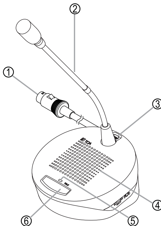
[TS-682L-AS Isometric]
