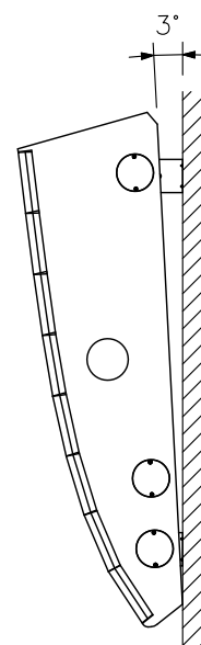
Mounting example (Downward angle: 3°) (scale: 1/20)
