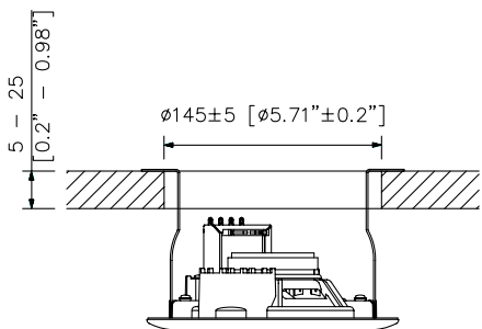
Mounting Diagram
