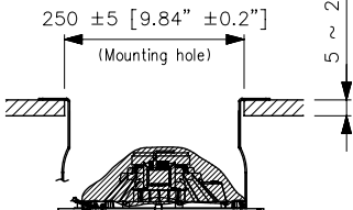
Mounting diagram (Scale 1/4)
