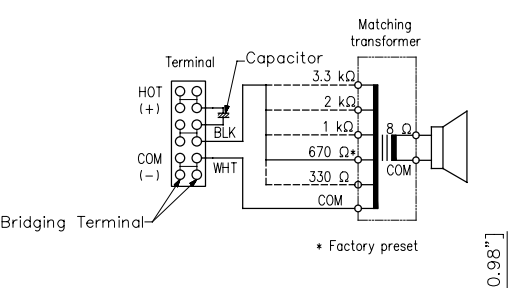
Wiring Diagram for PC-668RC:
