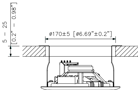
Mounting Diagram
