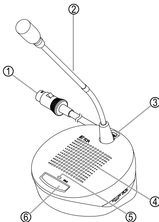
[TS-682L-AS Isometric]
