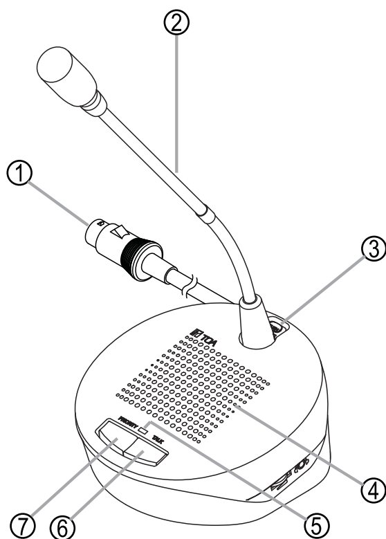
[TS-681L-AS Isometric]
