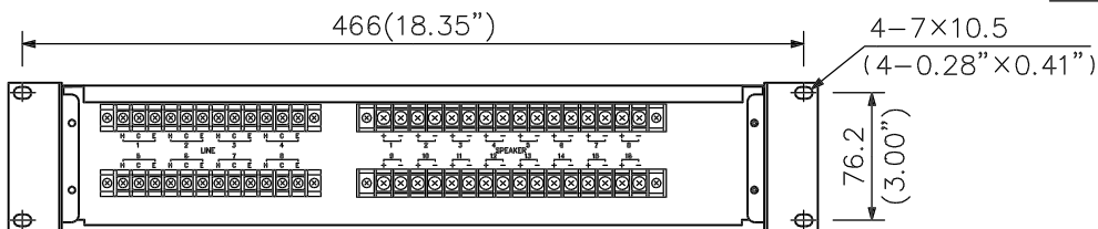
Front View Without Front Panel
